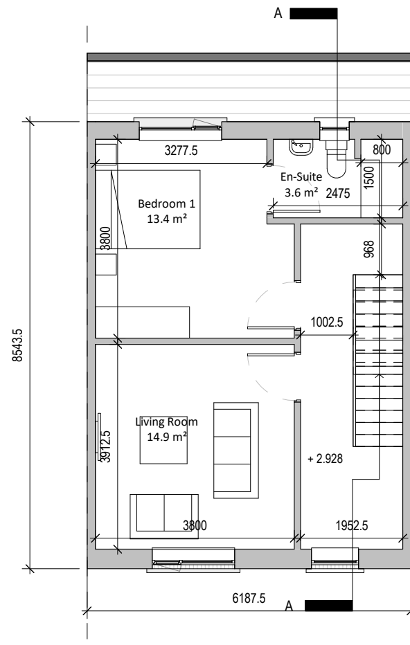
② First Floor Mid Terrace - Type A 1 : 100
