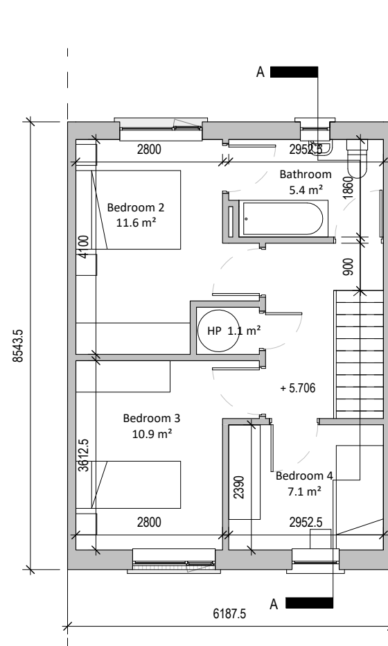
③ Second Floor Mid Terrace - Type A 1 : 100
