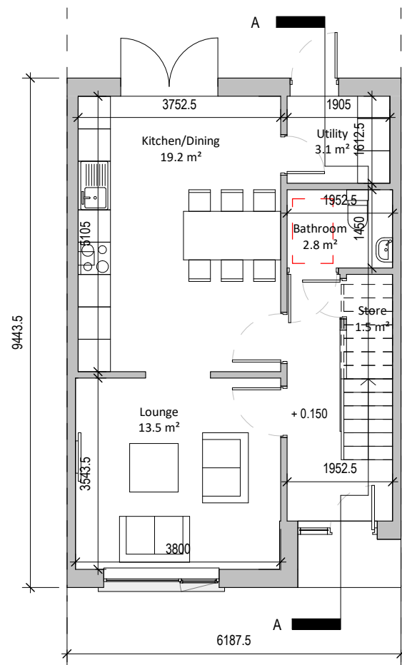
① Ground Floor Mid Terrace - Type A 1 : 100
