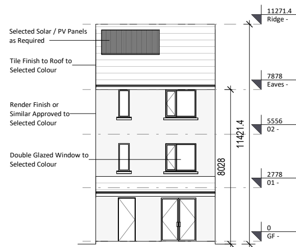
⑤ Rear Elevation - Type A 1 : 200
